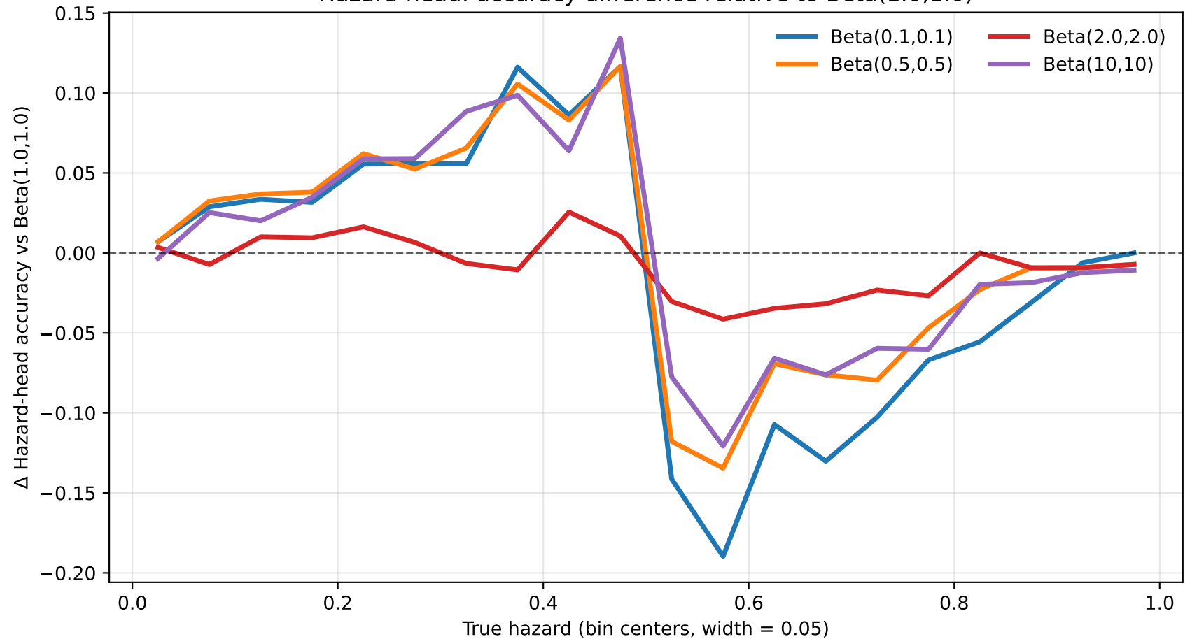
Hazard-head: accuracy difference relative to Beta(1.0,1.0)
